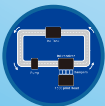
White Ink Recirculation System
